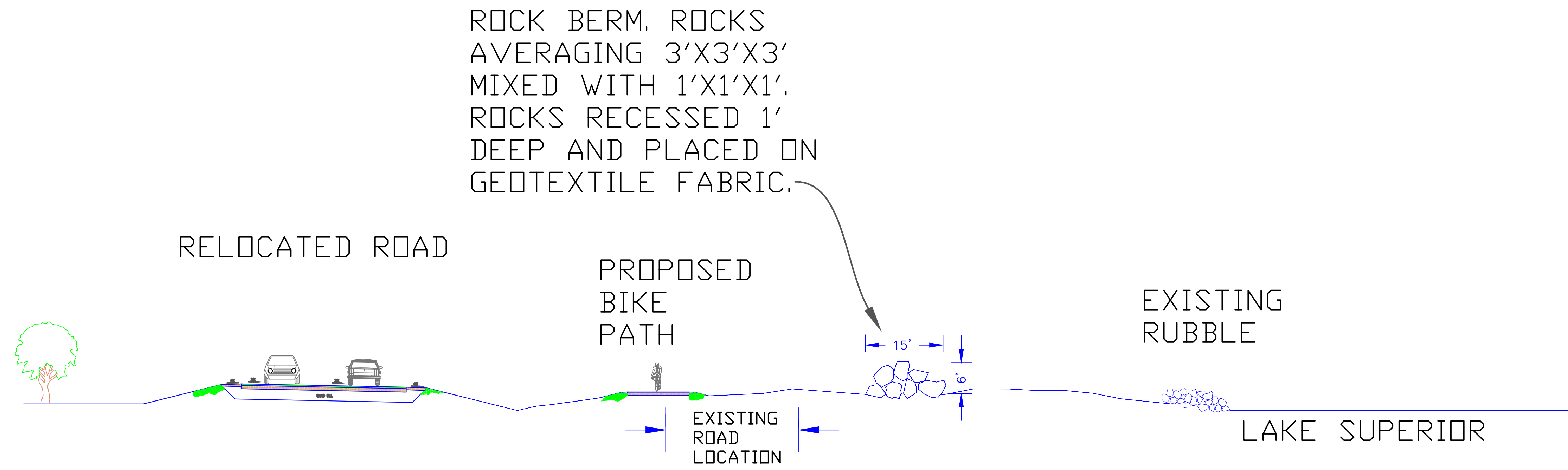
CROSS SECTION THROUGH NORTH END OF STONE BERM
