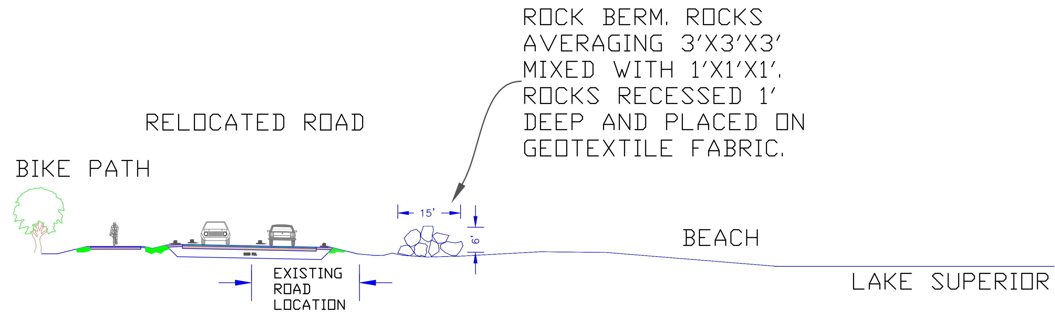
CROSS SECTION THROUGH SOUTH END OF STONE BERM
